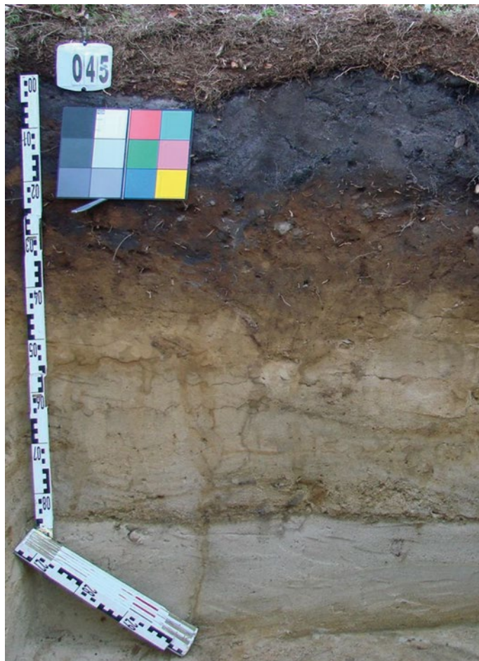
Braunerde-Podsol
